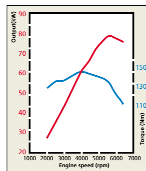
M16A engine performance curves
