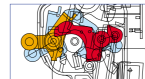
Side door lock mechanism (deadlock)
