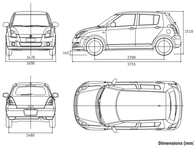
Dimensions (mm)
